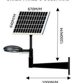
REF:BRZ-PREMIUN+URA D-21H-SL-09
