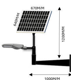
REF:BRZ-PREMIUN+BORA H9-SL-17
