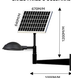
REF:BRZ-PREMIUN+ECA D-32 H9-SL-08
