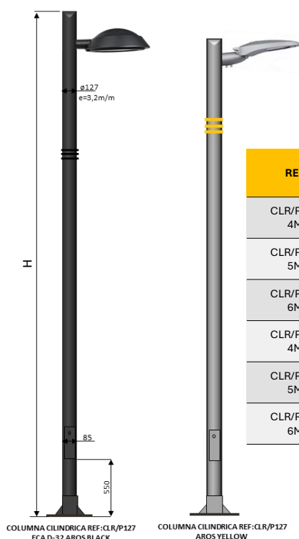
COLUMNA CILINDRICA REF: CLR/P127 ECA D-32 AROS BLACK COLUMNA CILINDRICA REF: CLR/P127 AROS YELLOW
