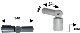
REF: RTL-LM-60ø
